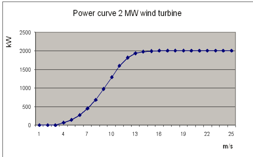
Figure 2a – Power curve of a 2 MW wind turbine (without noise reduction measures).
