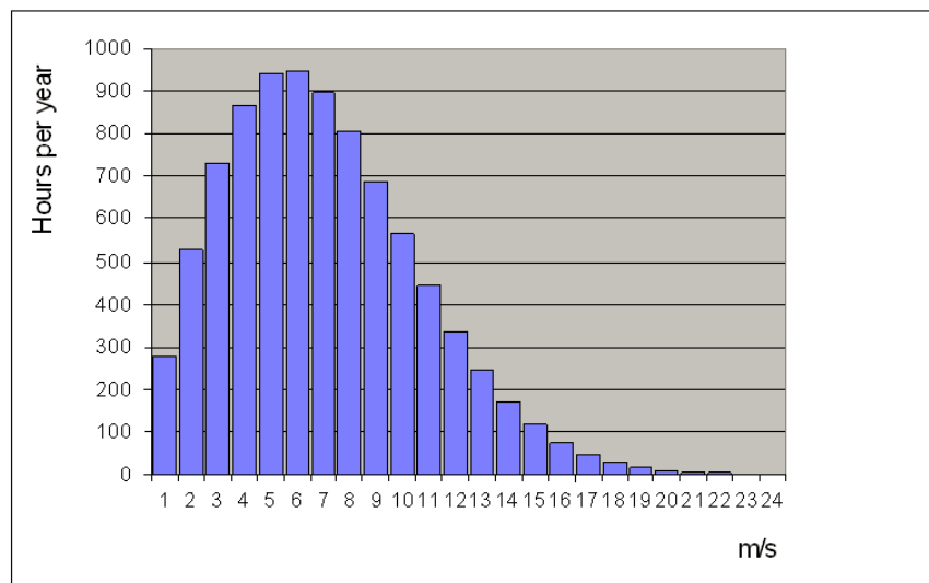
Figure 2b – Wind speed distribution, average wind speed 7.0 m/s and Weibull shape factor k=2.0 .
